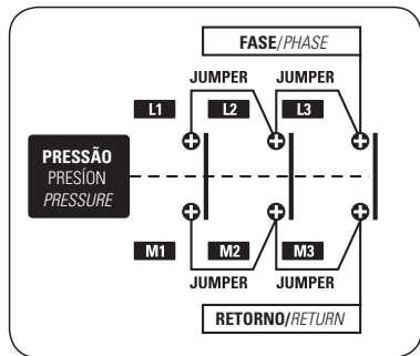
TRIFÁSICO THREE-PHASE
